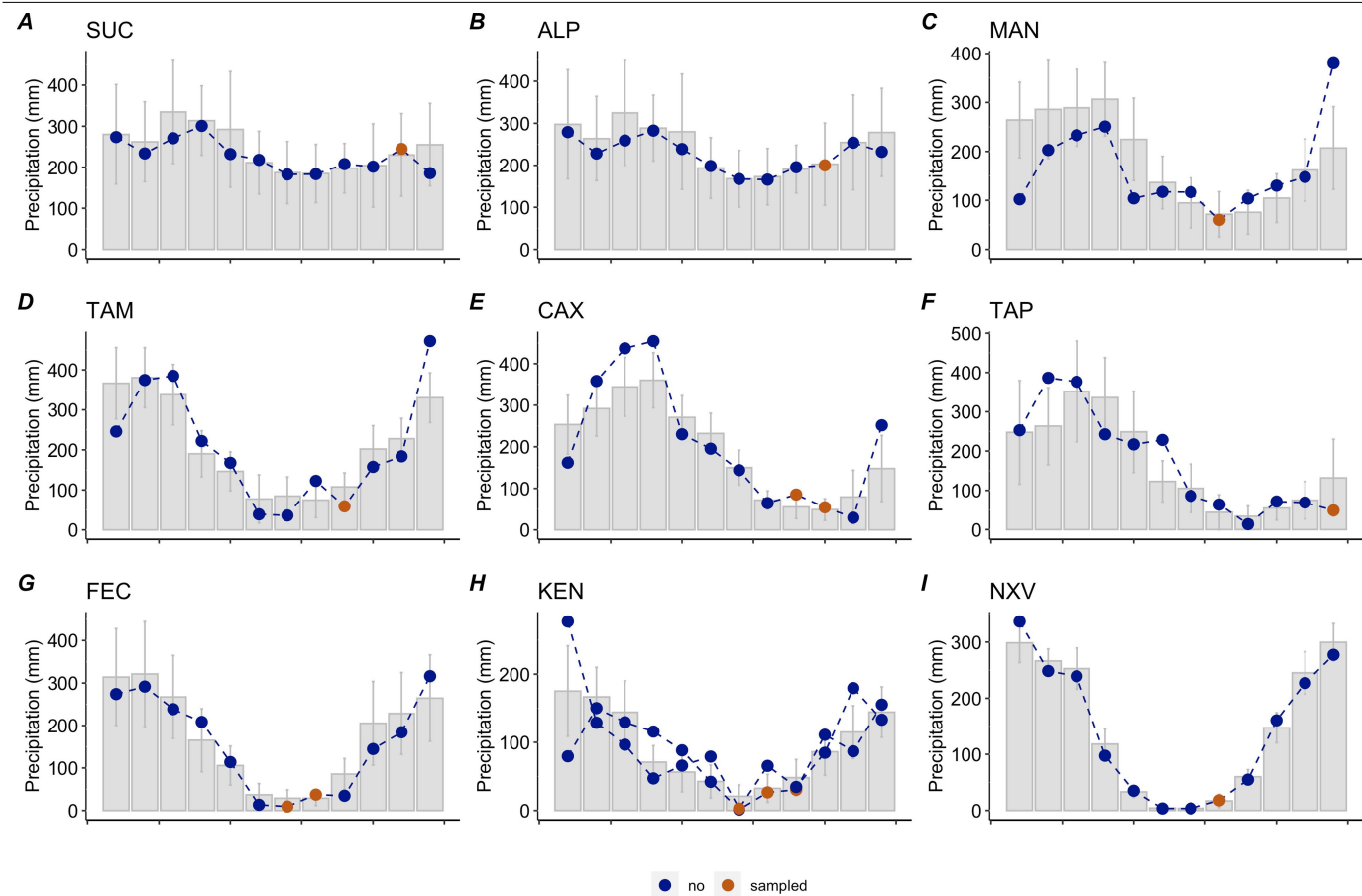
Extended Data Fig. 2 | Climatological data corresponding to \Psi_{dry} (in situ dry season leaf water potential) sampling at each site. Grey bars and error bars show the mean and standard deviation of monthly precipitation from 1991 to 2018 (CRU data ts.4.0338) 75 . The blue dashed lines represent the year of sampling, while the brown points show the months at which \Psi_{dry} was measured. Hydraulic
