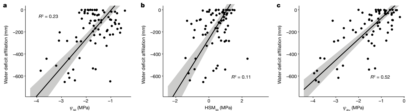
Fig. 3 | Relationship between WDA and HTs across western Amazon tree species. a–c, Embolism resistance \psi_{50} ( a ), hydraulic safety margin HSM_{50} ( b ) and minimum leaf water potential observed in the dry season \psi_{dry} ( c ). Individual points indicate species mean trait values ( n = 87 ). Less negative WDA values denote wet-affiliated species and more negative WDA denote
