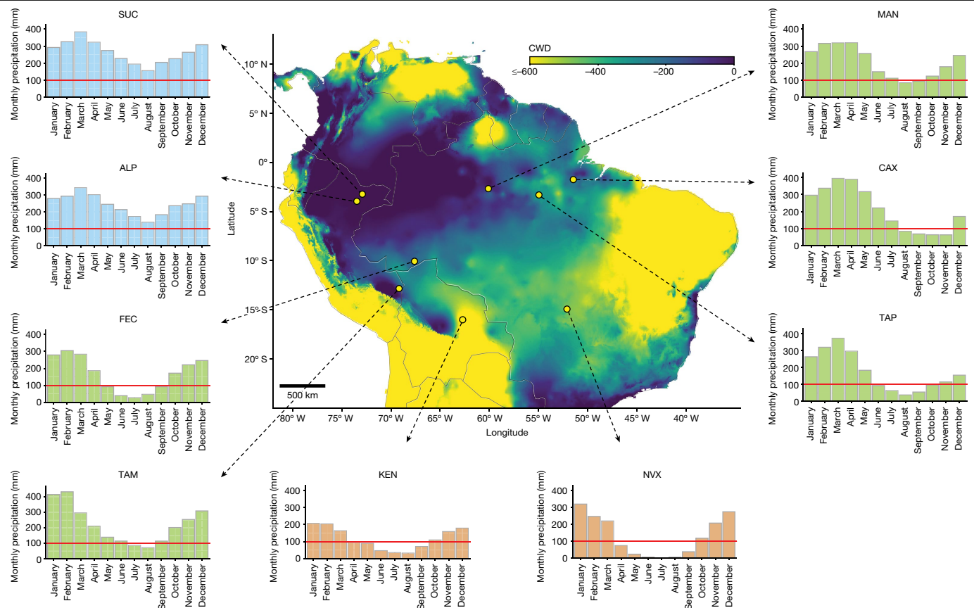
Fig. 1 | Sampled sites: spatial distribution and climatological variation.
