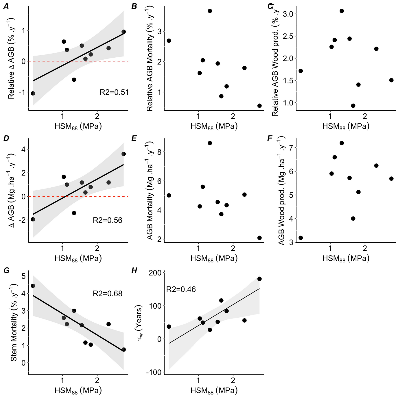
Extended Data Fig. 10 | HSM 88 Plot-level analyses: bivariate relationships between basal area-weighted mean HSM 88 and forest dynamics across Amazonian forest plots. Basal area-weighted mean HSM 88 in relation to relative (A-C) and absolute (D-H) forest dynamics values. A) Relative annual aboveground biomass net change ( \Delta AGB/AGB), where: \Delta AGB is the difference in aboveground biomass between the final and initial censuses ( AGB_{\text{final census}} - AGB_{\text{initial census}} ) divided by total monitoring length for that plot ( \text{Date}_{\text{final census}} - \text{Date}_{\text{initial census}} ) in years and AGB is the time-weighted mean standing woody biomass across censuses per plot; B) Relative annual mortality in terms of biomass: ( AGB_{\text{MORT}}/AGB ). Where AGB_{\text{MORT}} is the sum of the AGB of all dead trees and the unobserved components (see methods), divided by the census interval length 95 ; C) Relative annual AGB wood productivity: ( AGWP/AGB ), where AGWP is defined as the sum of the biomass growth of surviving trees >10 cm DBH, new recruits >10 cm DBH and the unobserved components
