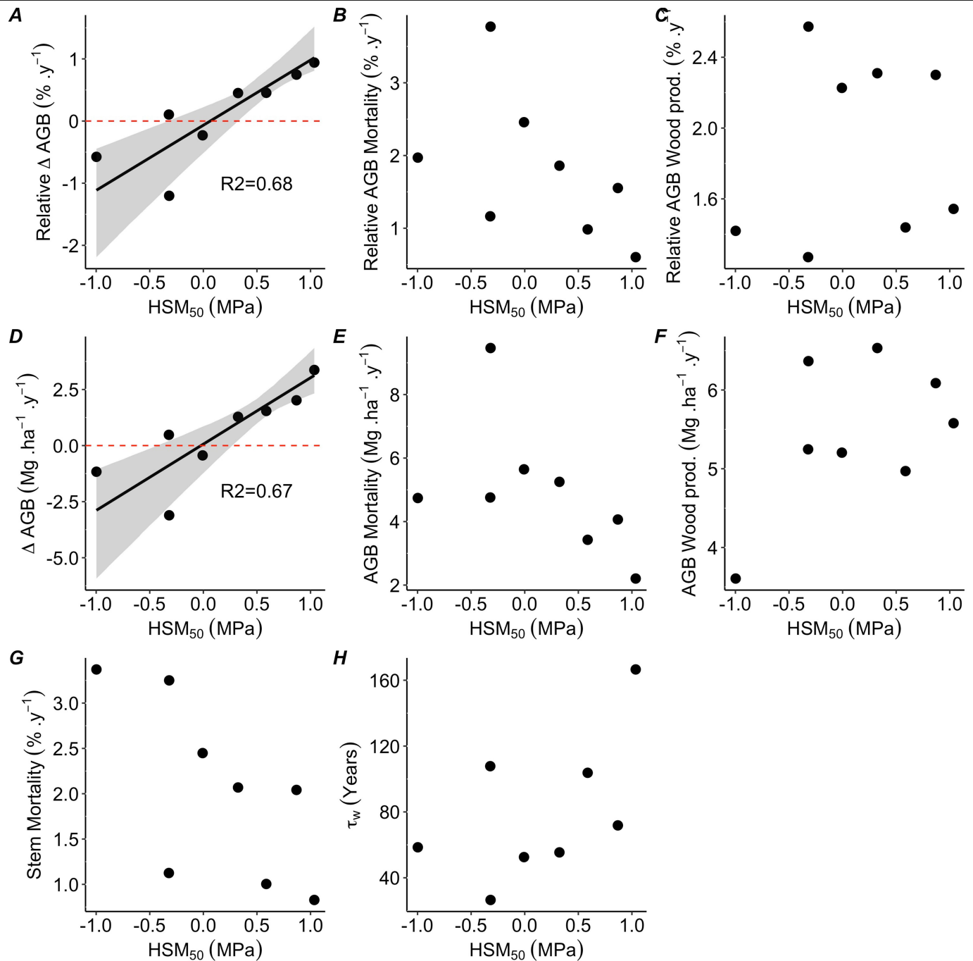
Extended Data Fig. 8 | Cluster-level analyses: Relationship between basal area weighted mean HSM 50 and cluster mean forest dynamics across clusters of forest plots. Basal area-weighted mean HSM 50 in relation to cluster mean relative (A–C) and absolute (D–H) forest dynamics values. A) Relative annual aboveground biomass net change ( \Delta AGB/AGB), where: \Delta AGB is the difference in aboveground biomass between the final and initial censuses ( AGB_{final\ census} - AGB_{initial\ census} ) divided by total monitoring length for that plot ( Date_{final\ census} - Date_{initial\ census} ) in years and AGB is the time-weighted mean standing woody biomass across censuses per plot; B) Relative annual mortality in terms of biomass: ( AGB_{MORT}/AGB ). Where AGB_{MORT} is the sum of the AGB of all dead trees and the unobserved components (see methods), divided by the census interval length 95 ; C) Relative annual AGB wood productivity: ( AGWP/AGB ), where AGWP is defined as the sum of the biomass growth of surviving trees >10 cm DBH, new recruits >10 cm DBH and the unobserved components
